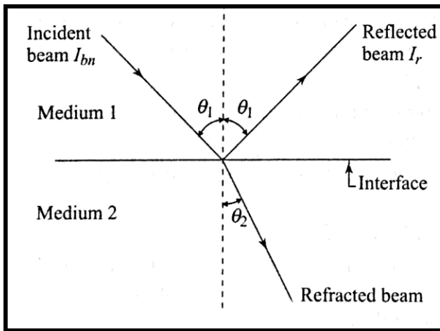
Fig. Reflection and Refraction at the interface of two media
