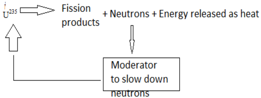
Fig. Fission reaction of U^{235}
