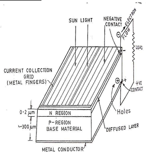
Fig. 5.6.1. Schematic view of a typical solar cell.
