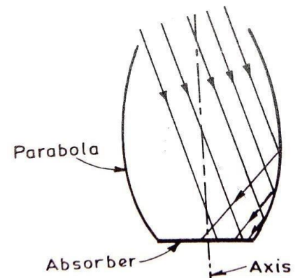
Fig. 3.7.10. Compound parabolic concentrator.
