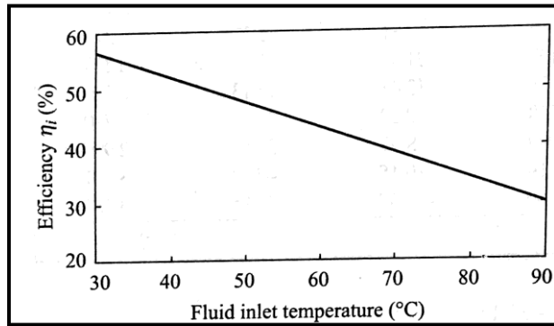
fig.: Variation of efficiency of a collector with fluid inlet temperature
