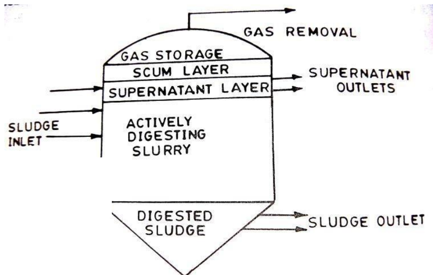
Fig. 7.6.1. Schematic of single process conventional digester.
