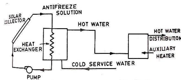
Fig. 5.2.5. Solar water heating system with antifreeze.
