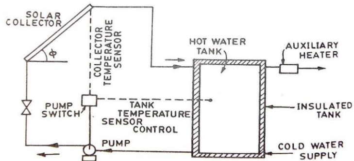
Fig. 5.2.4. Schematic of a forced circulation solar water heater.
