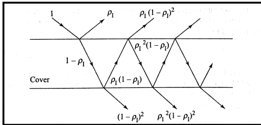
Fig.: Ray diagram showing transmission through a single cover considering reflection - refraction
