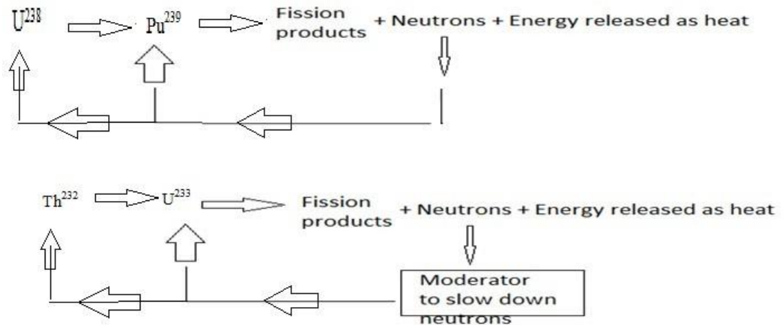
Fig.13. Breeder reactor for U^{238} & Th^{232}
