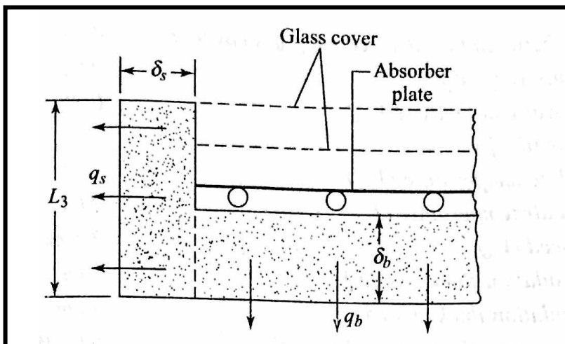
Fig.: Bottom and Side Losses from a flat plate collector
