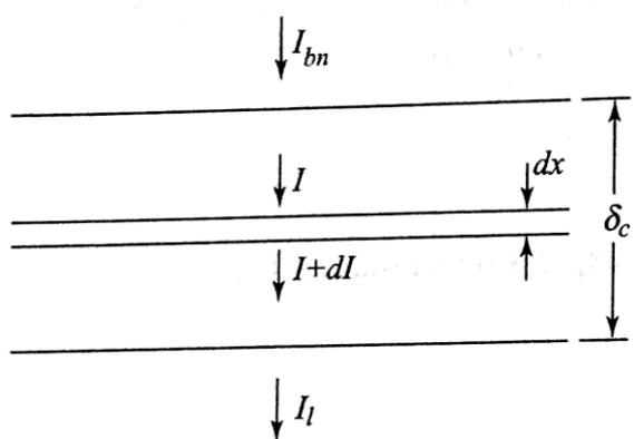
Fig.: Absorption in a transparent cover
