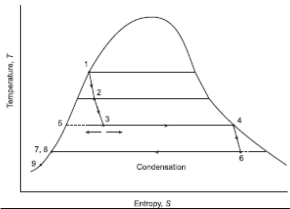
Single flash, wet steam high temperature hydrothermal system
