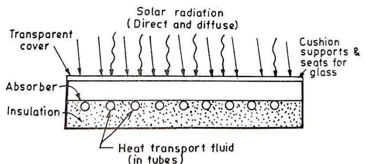
Fig. 3.3.1. Selection through typical flat-plate collector.
