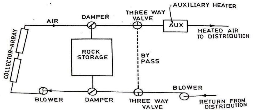
Fig. 5.3.6. Schematic diagram of a basic hot air heating system.
