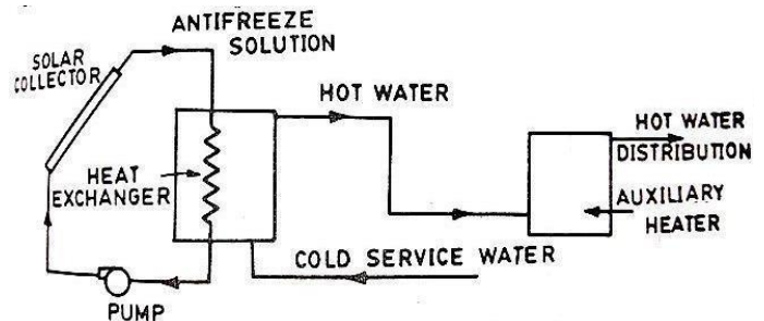
Fig. 5.2.5. Solar water heating system with antifreeze.
