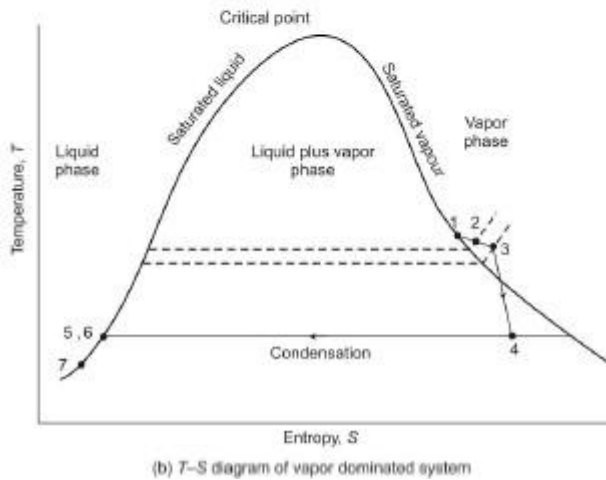
Figure: Dry steam hydrothermal system
