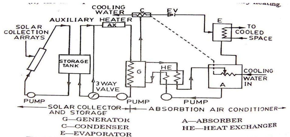
Fig. 5.4.1. Schematic of Solar Operated Absorption Air Conditioner.
