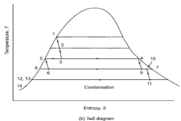
Double flash, wet steam high temperature hydrothermal system
