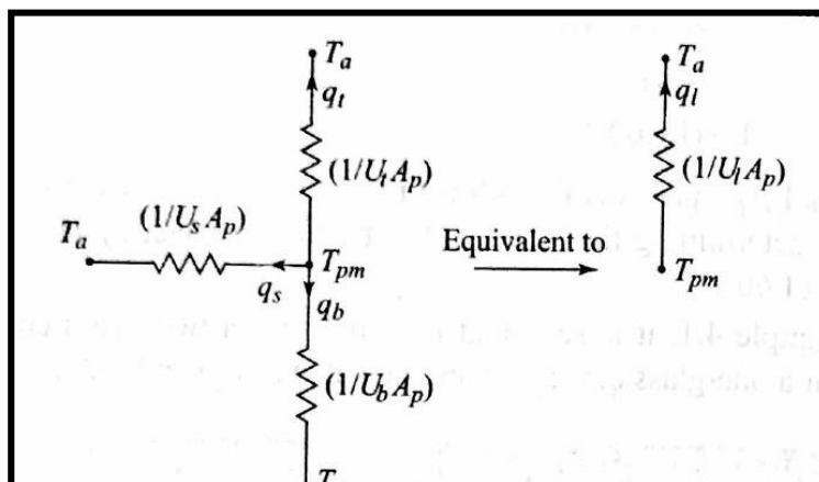
Fig.: Thermal Resistance Network showing collector losses
