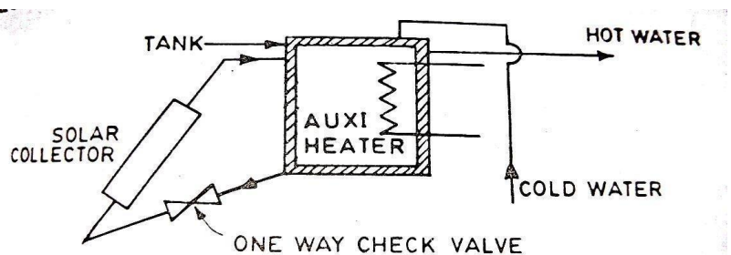
Fig. 5.2.2. Non-pressurized solar water heater.
