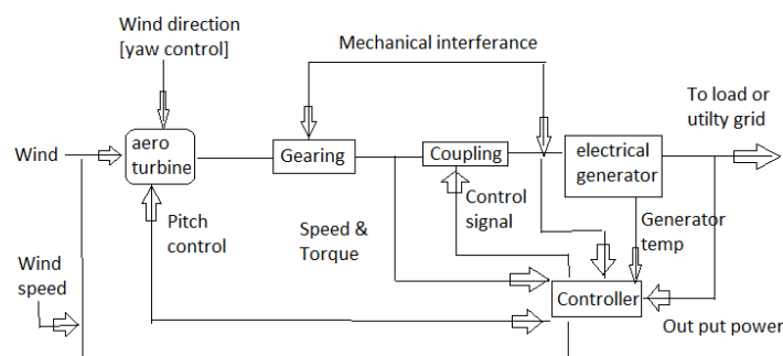
Fig Basic components of wind electric system
