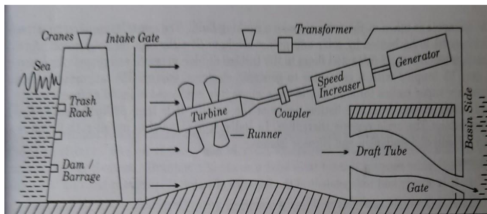
Fig: 4.5: Schematic layout of tidal power house
