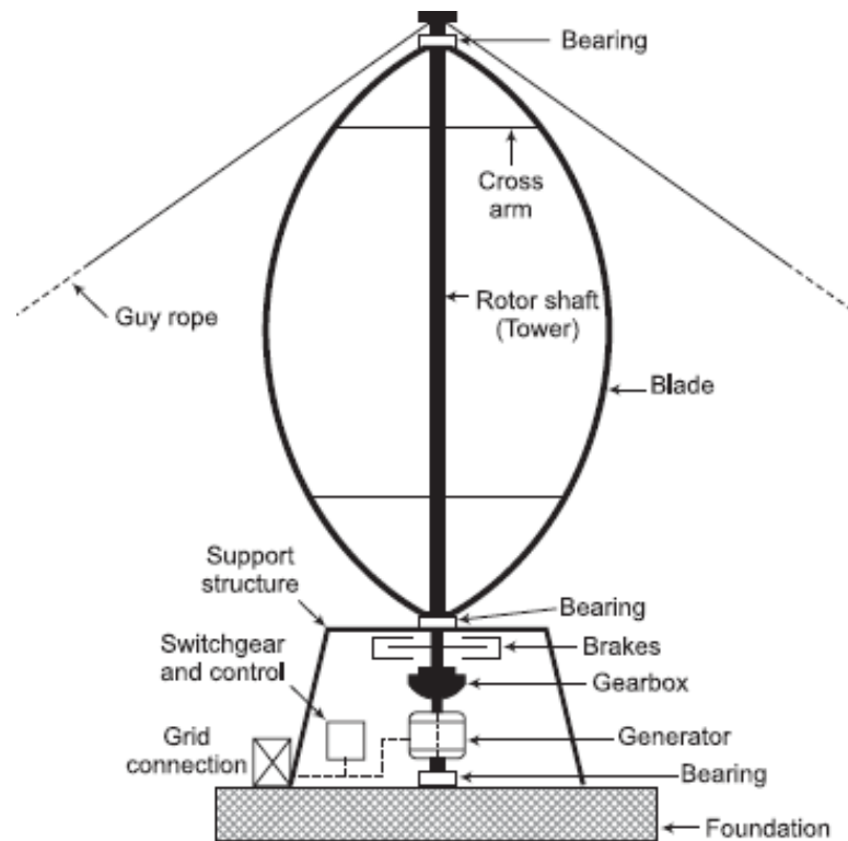
Fig 4.1: Vertical axis Darrieus wind turbine
