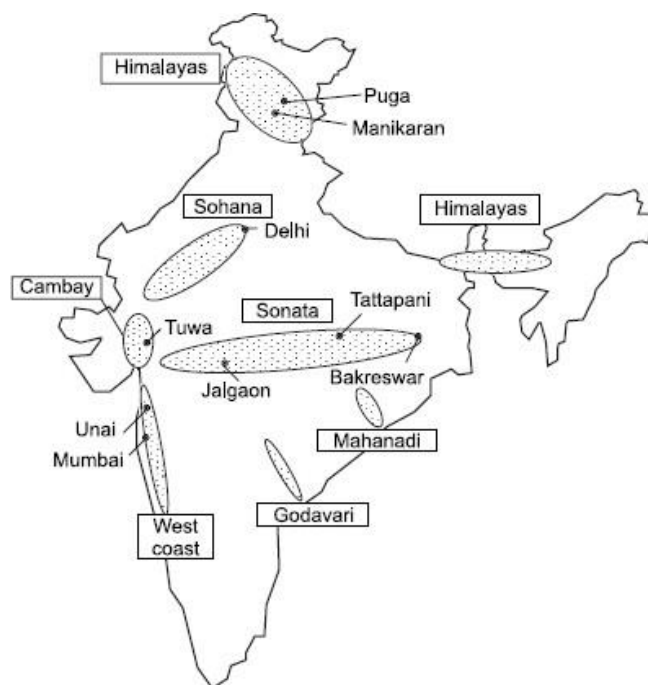
Figure Geothermal provinces of India (not to scale)
