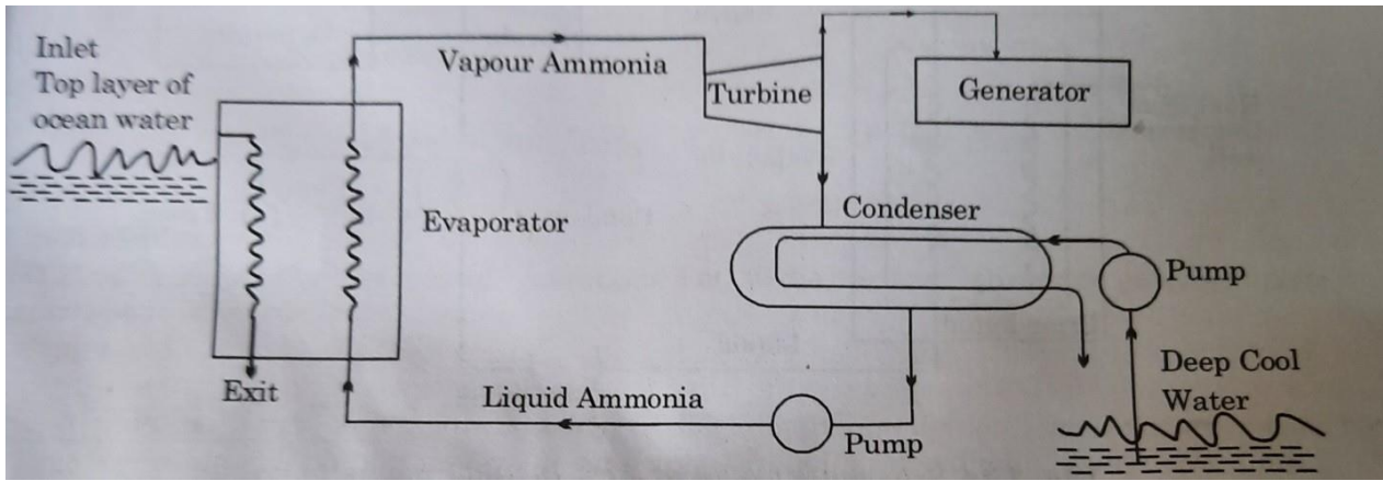
Fig 4.6: Ocean thermal energy conversion – open cycle system
