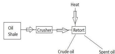
Production of crude oil from oil shale
