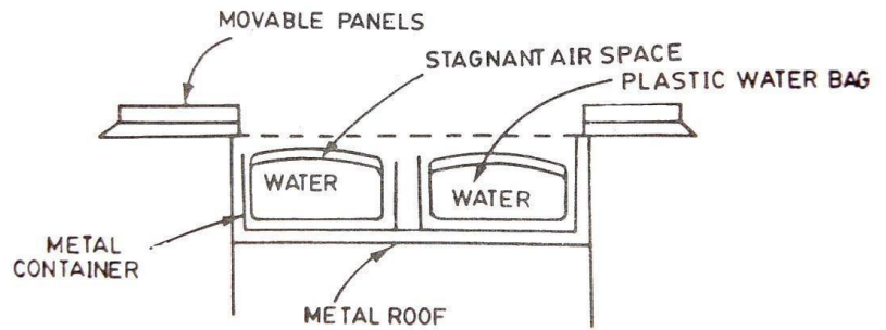
Fig. 5.3.2. Roof storage of Solar heat.
