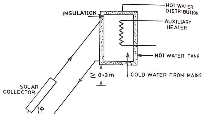
Fig. 5.2.1. Schematic of a neutral circulation solar water heater (pressurized).
