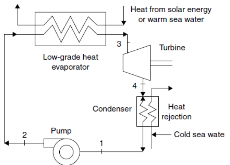
Fig 4.7: OTEC Rankine Cycle
